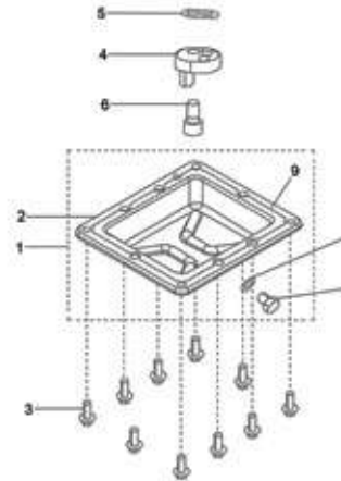
PLATE-8 OIL PAN Page No. :15-16
