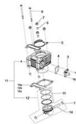
PLATE-16 Cylinder- Piston Group
