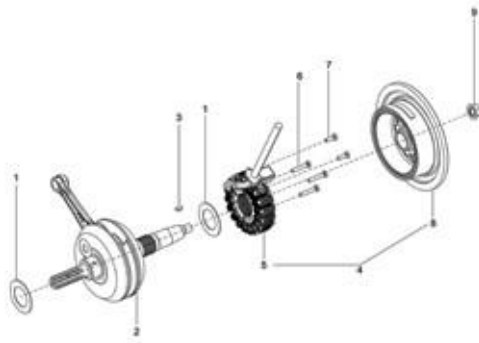
PLATE-15 Timing Group
