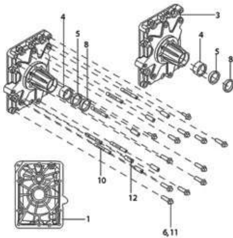
PLATE-7 OIL FILTER & PRESSURE RELIEF VALVE Page No. :13-14
