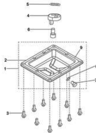
PLATE-8 OIL PAN Page No. :15-16
