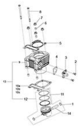
PLATE-15 Cylinder- Piston Group
